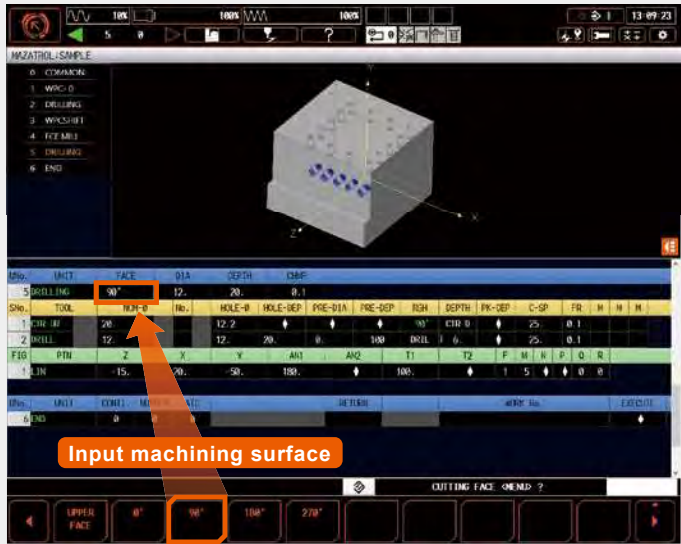
Coordinate system and machining surface
