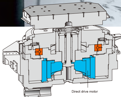
Direct drive motor/table cross section
