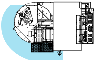
2 pallet changer ■ : Operation area
